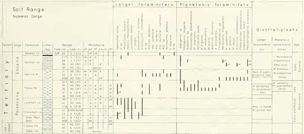
Fig. 3: Distribution of larger and planktonic foraminifers of the Namgal Gorge section, western Salt Range. Abbreviations see Fig. 2.
